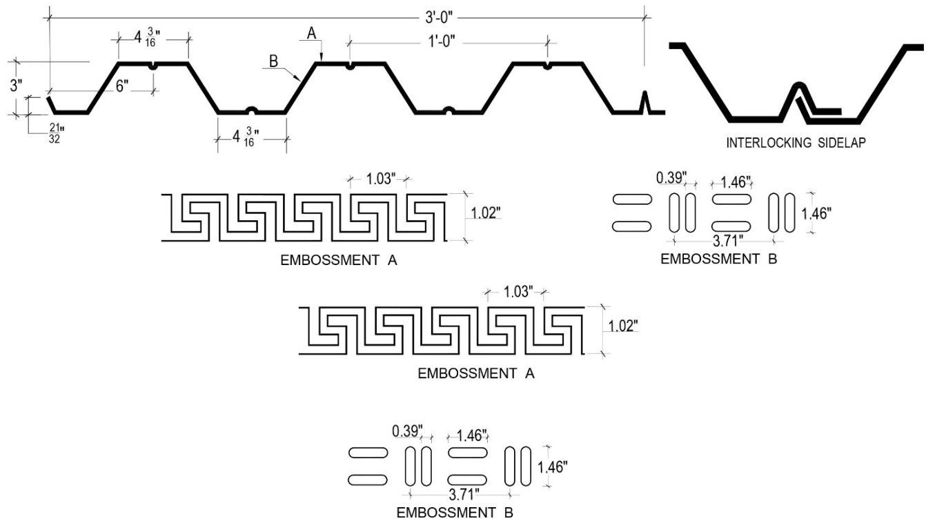
figure 4 3X12 FLOOR DECK
