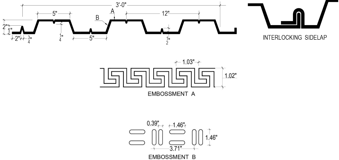
figure 3 2 X 12 FLOOR DECK
