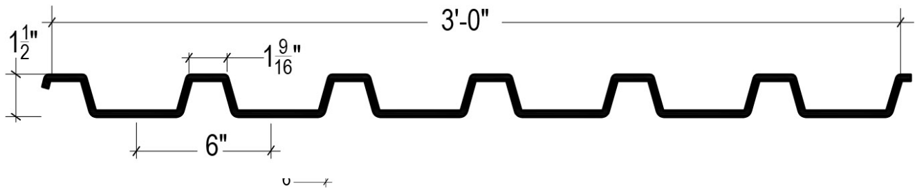
figure 5 1½ X 6 INV FLOOR DECK
